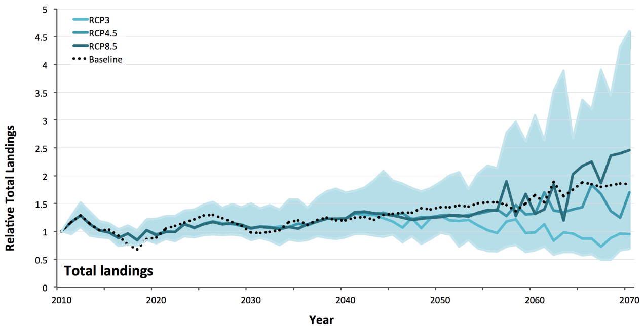
Figure 30: Average relative total landings through time from Atlantis-SE under each emission scenarios. The lighter shaded area is the total range.
