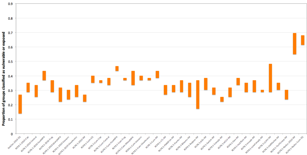
Figure 26: Range of proportion of the groups classified as vulnerable or exposed in 2065-2070 in Atlantis SE under RCP 8.5
