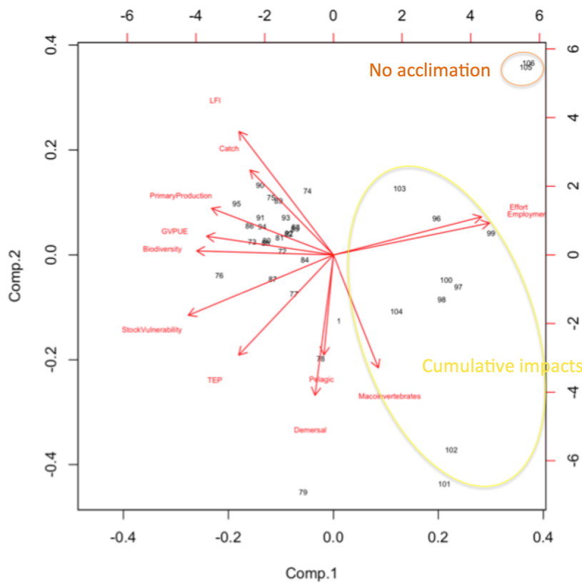
Figure 64: PCA biplot for Atlantis-SEAP simulations strategies and scenarios under RCP 8.5. Small numbers are IDs for individual strategy-scenario combinations.
