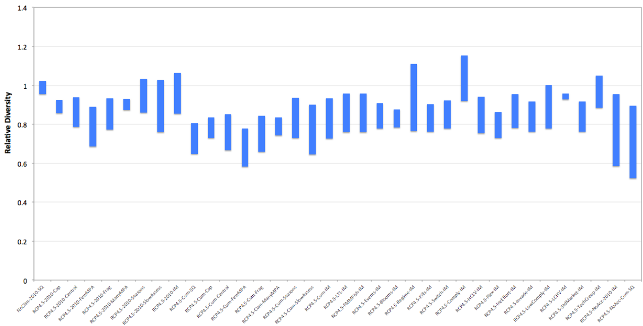
Figure 28: Range of relative marine biodiversity in 2065-2070 in Atlantis SE under RCP 4.5
