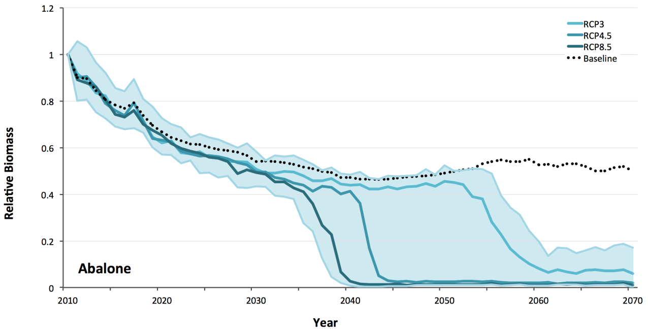
Figure 47: The average relative biomass of abalone through time in Atlantis-SEAP under the different emission scenarios. The lighter shaded area is the total range.
