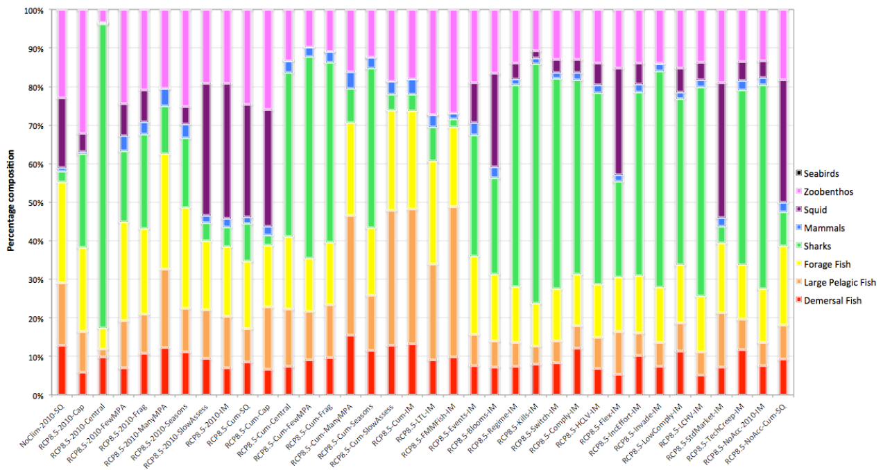
Figure 20: Average relative composition of biomass (2065-2070) across scenarios and strategies in Atlantis SE under RCP 8.5
