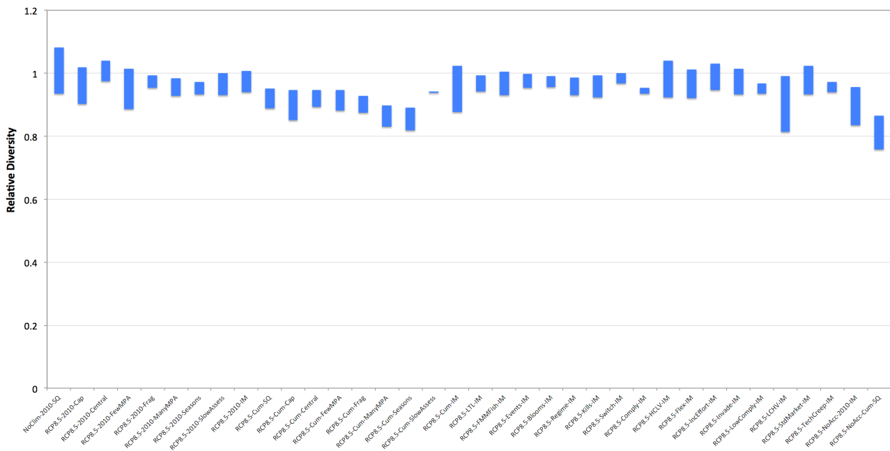
Figure 56: Range of relative marine biodiversity in 2065-2070 in Atlantis SEAP under RCP 8.5
