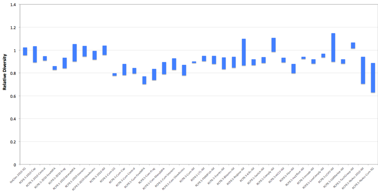
Figure 29: Range of relative marine biodiversity in Atlantis SE under RCP 8.5
