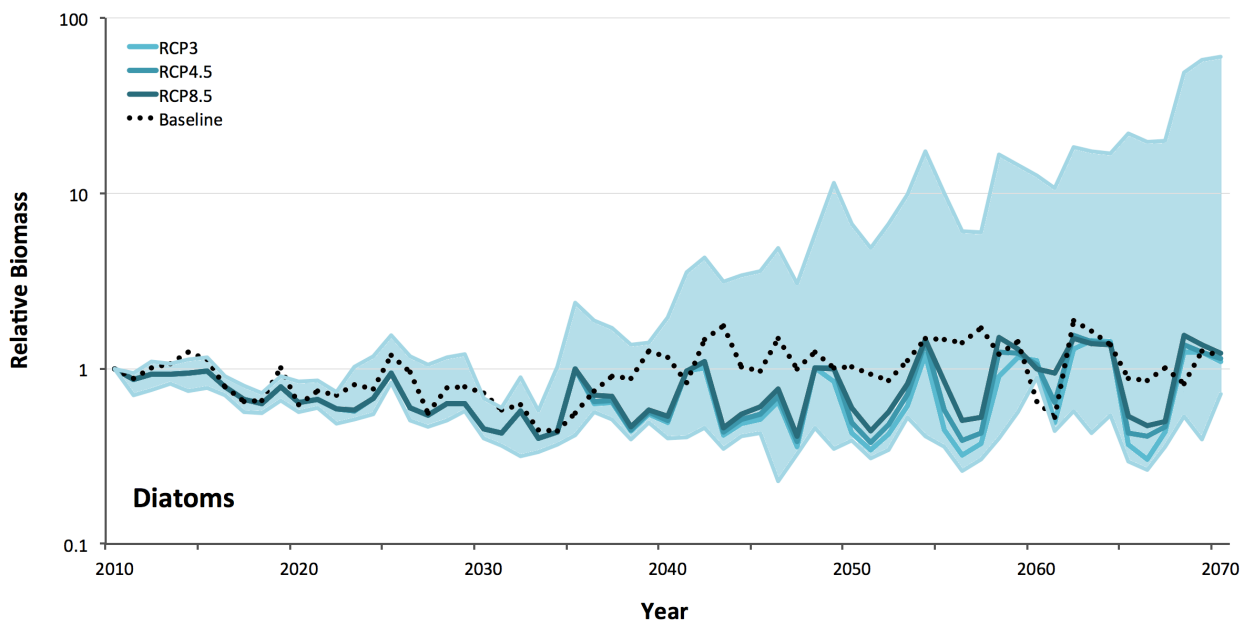
Figure 21: The average relative biomass of diatoms through time in Atlantis-SE under the different emission scenarios. The lighter shaded area is the total range.
