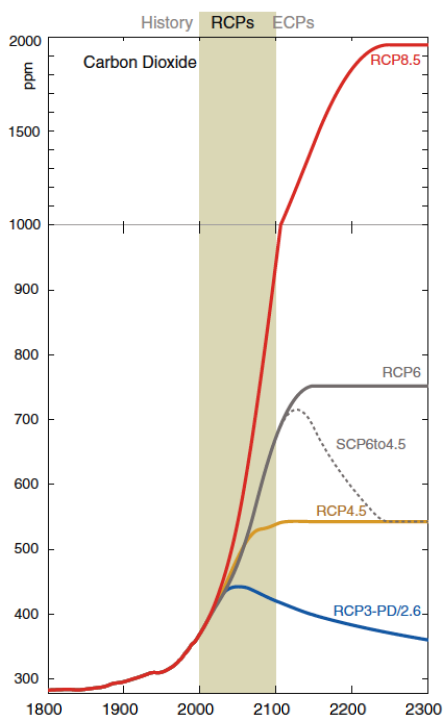
Figure 10: Atmospheric carbon content in the RCP scenarios (form Meinshausen et al 2011)
