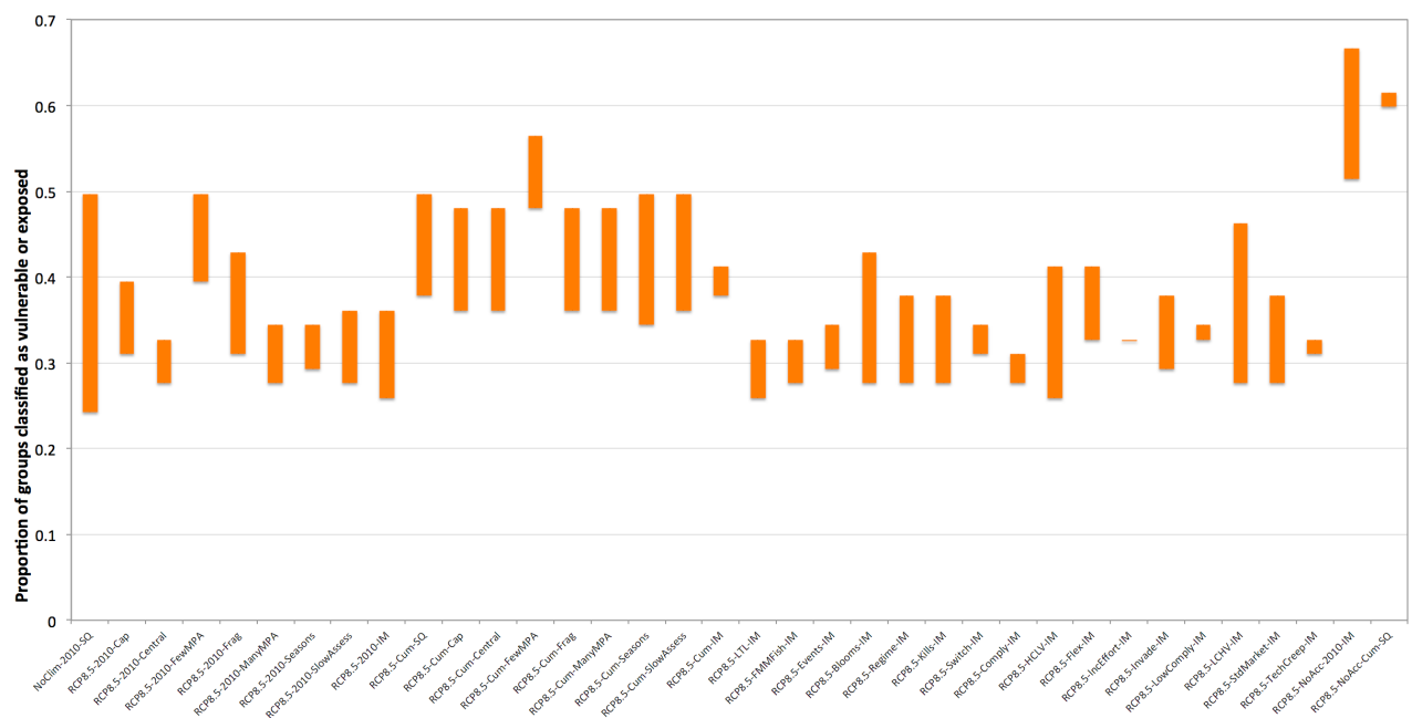
Figure 53: Range of proportion of the groups classified as vulnerable or exposed in 2065-2070 in Atlantis SEAP under RCP 8.5
